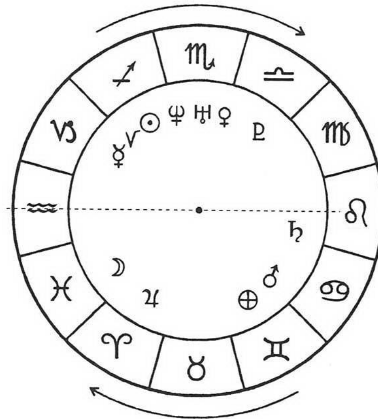
Clockwise movement of Signs around the Earth
