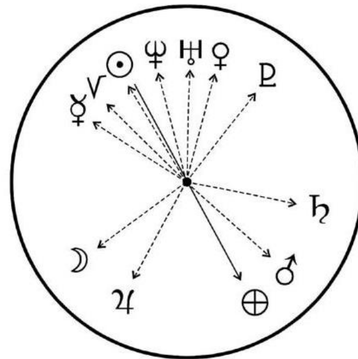
The Same Positions of the Planets Symbolised in the Horoscope geocentric, except for the earth itself, which is heliocentric and directly opposite the Sun
