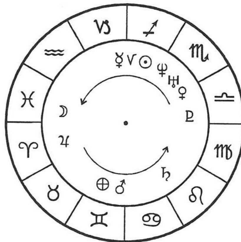
Anticlockwise movement of planets through the Signs
